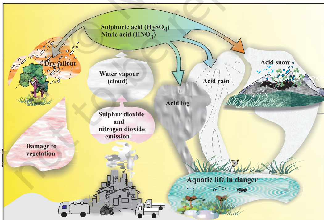
Fig. 14.1 Acid deposition
