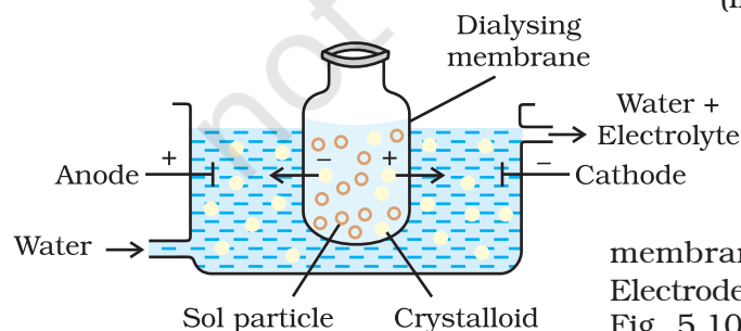
Fig. 5.10: Electro-dialysis
