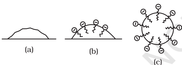
Fig. 5.7: (a) Grease on cloth (b) Stearate ions arranging around the grease droplet and (c) Grease droplet surrounded by stearate ions (micelle formed)
