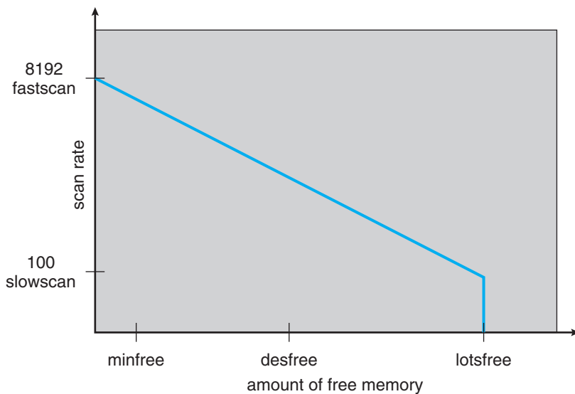
Figure 10.30 Solaris page scanner.
