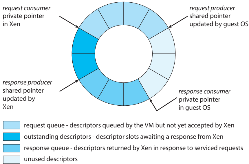
Figure 18.6 Xen I/O via shared circular buffer. 1
