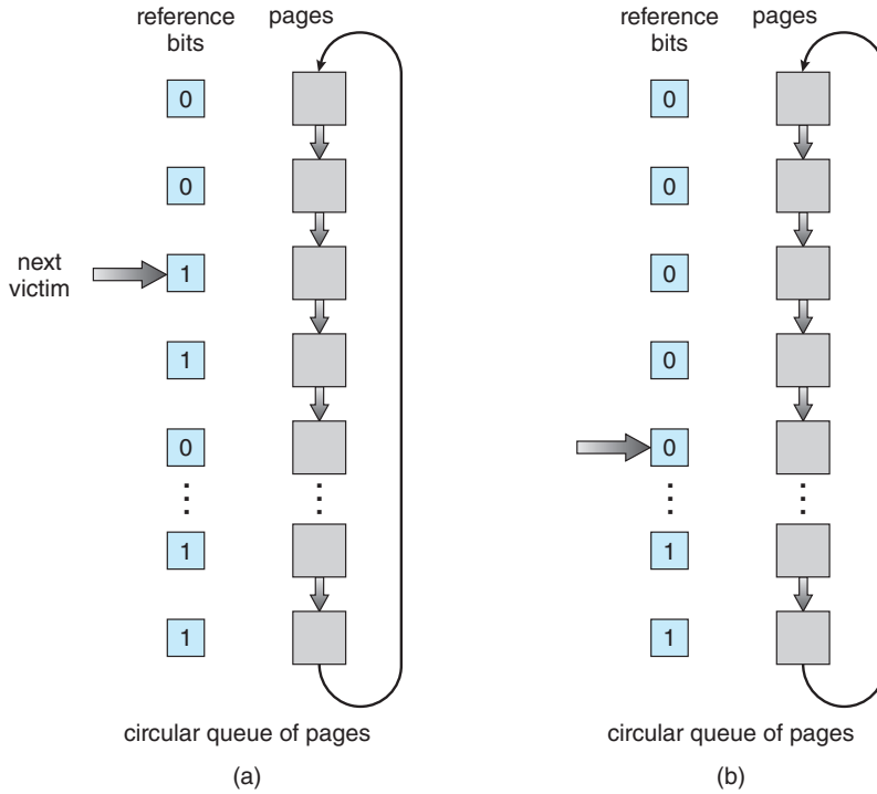
Figure 10.17 Second-chance (clock) page-replacement algorithm.
