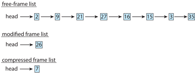
Figure 10.25 Free-frame list after compression
