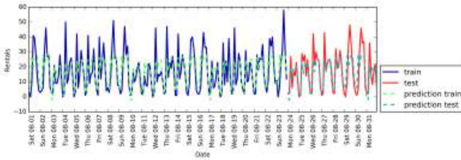
Figure 4-17. Predictions made by linear regression using a one-hot encoding of hour of day and day of week
