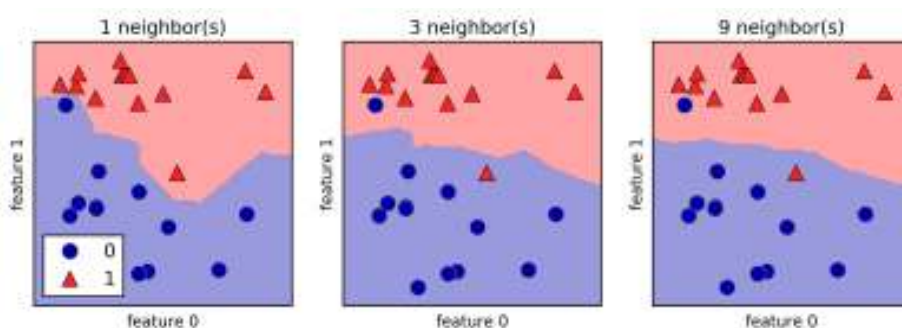
Figure 2-6. Decision boundaries created by the nearest neighbors model for different values of n\_neighbors
