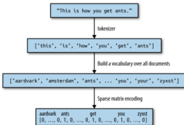
Figure 7-1. Bag-of-words processing
