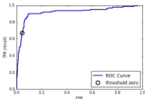
Figure 5-15. ROC curve for SVM
