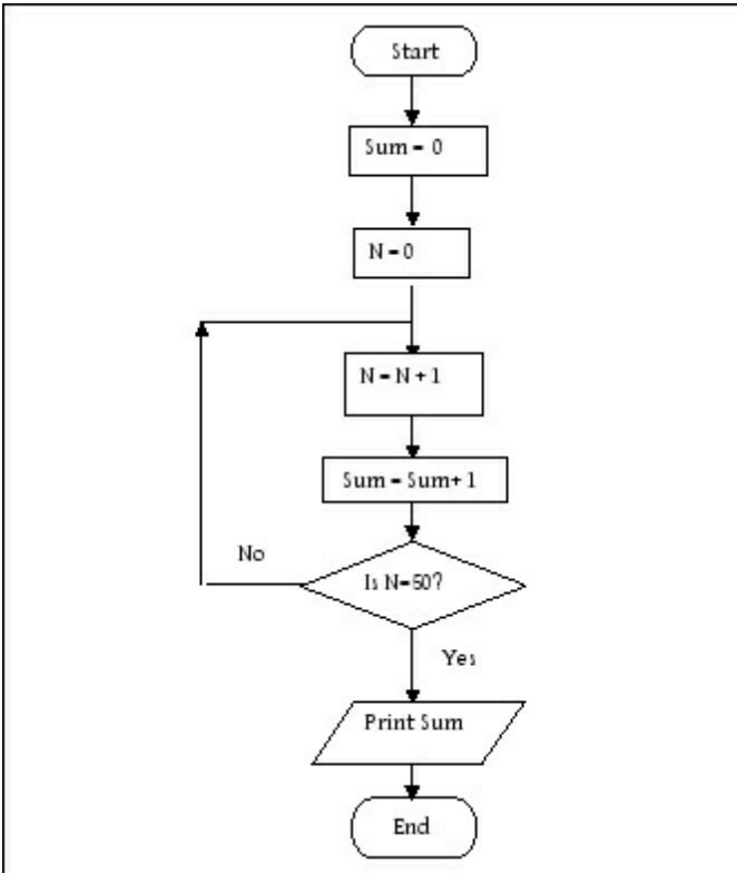
Sum of first 50 natural numbers
