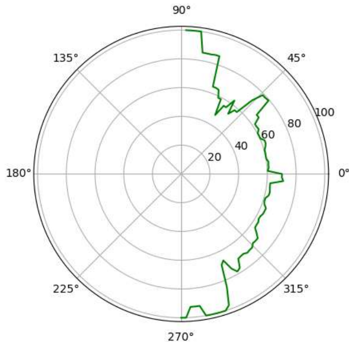
Figure 10.23 – A sonar scan plot of my lab
