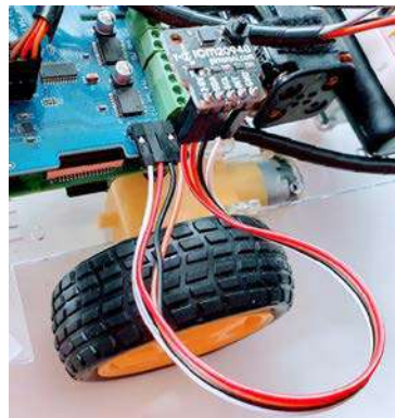
Figure 12.11 – ICM20948 IMU wired to the motor board
