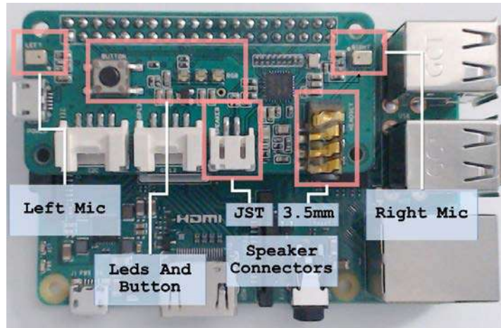
Figure 15.1 – The ReSpeaker 2-Mics Pi HAT
