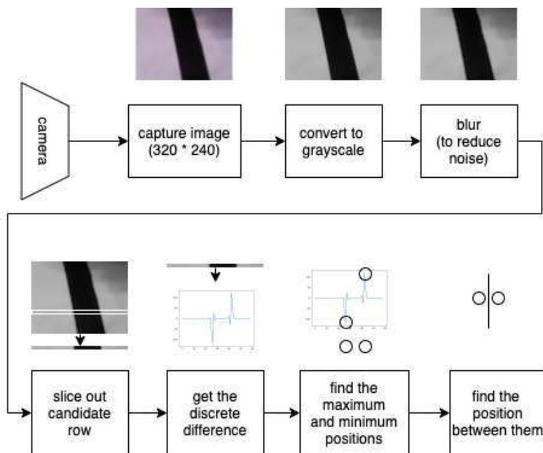
Figure 14.6 – Image processing pipeline for finding a line
