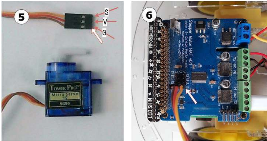
Figure 10.6 – Plugging a servo into the control board
