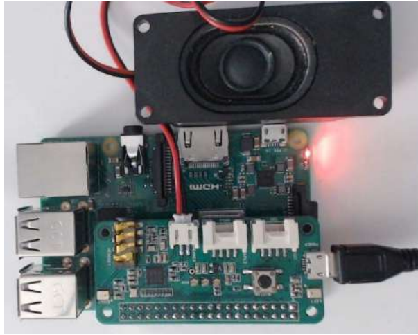
Figure 15.2 – The Mycroft Voice Assistant ReSpeaker setup
